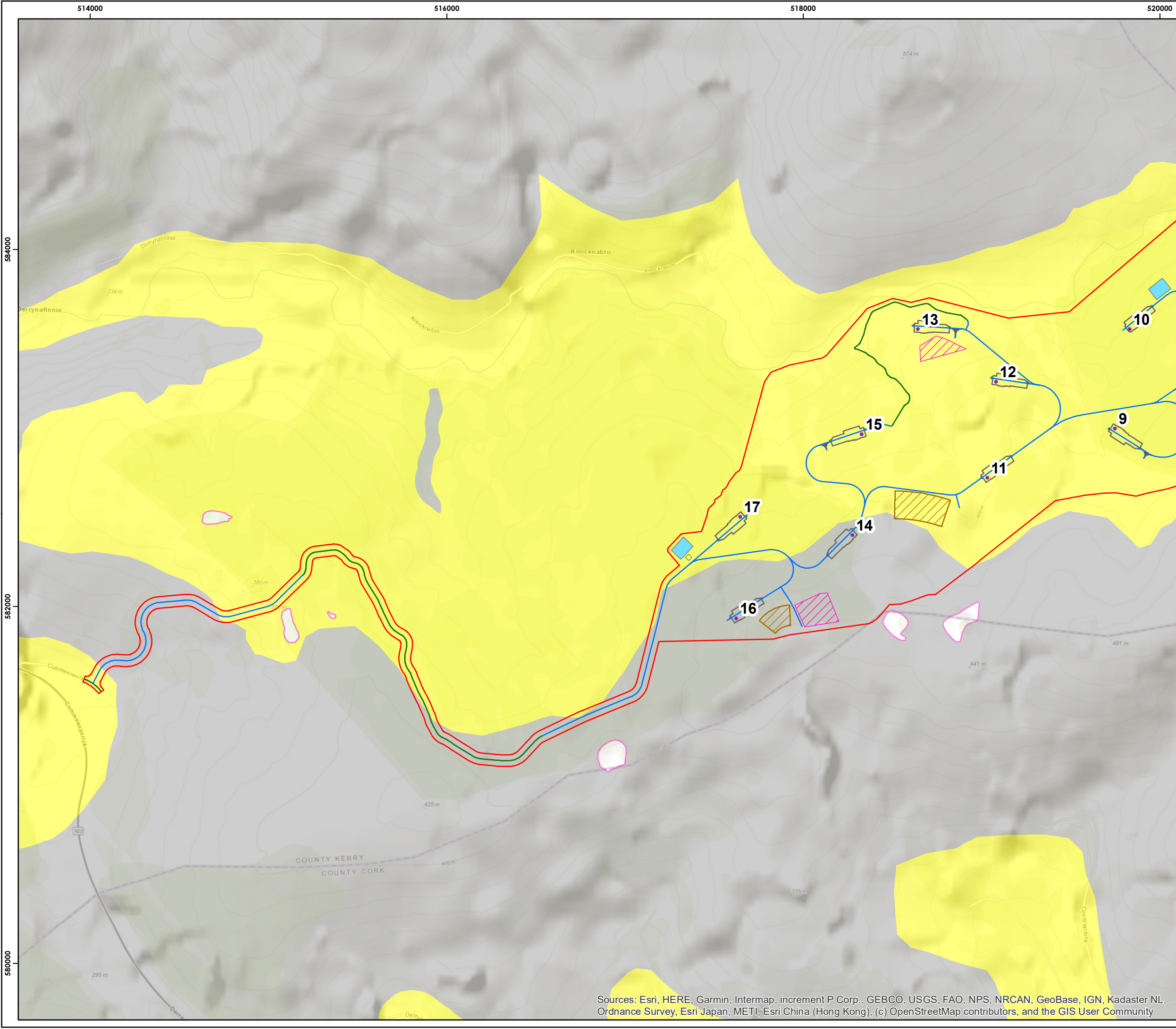
Figure10-6a Subsoil Permeability
